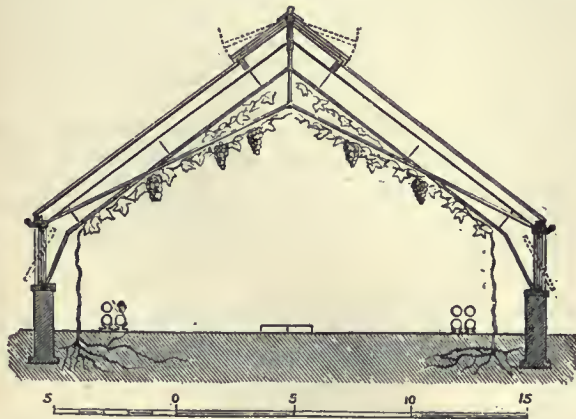
FIG. 7.—Span-Roofed Vinery.
